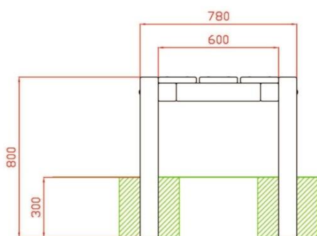
Vista Frontal
