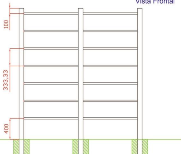
Vista Frontal
