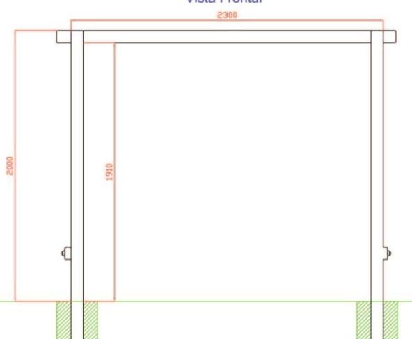
Vista Frontal
