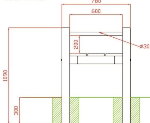
Vista Frontal
